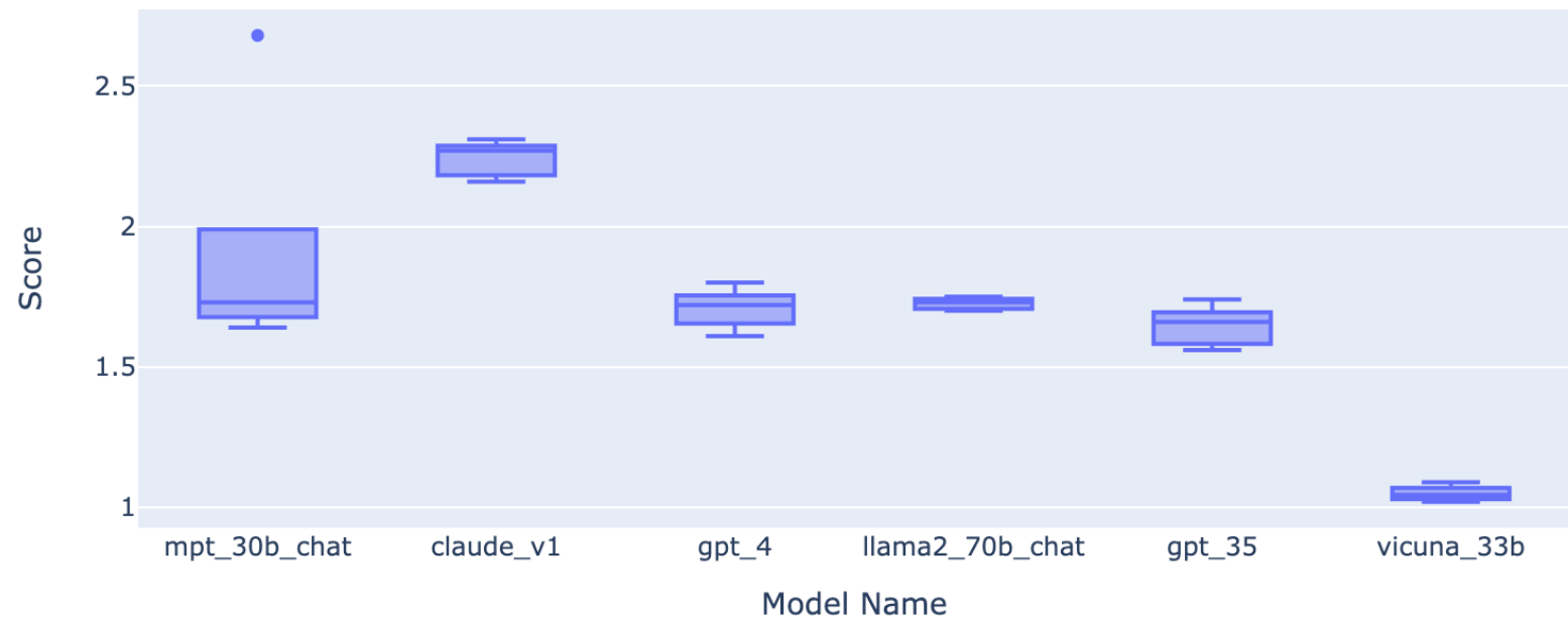
gpt-3.5-turbo-16k as Judge: LLM Score Variation: Zero shot
